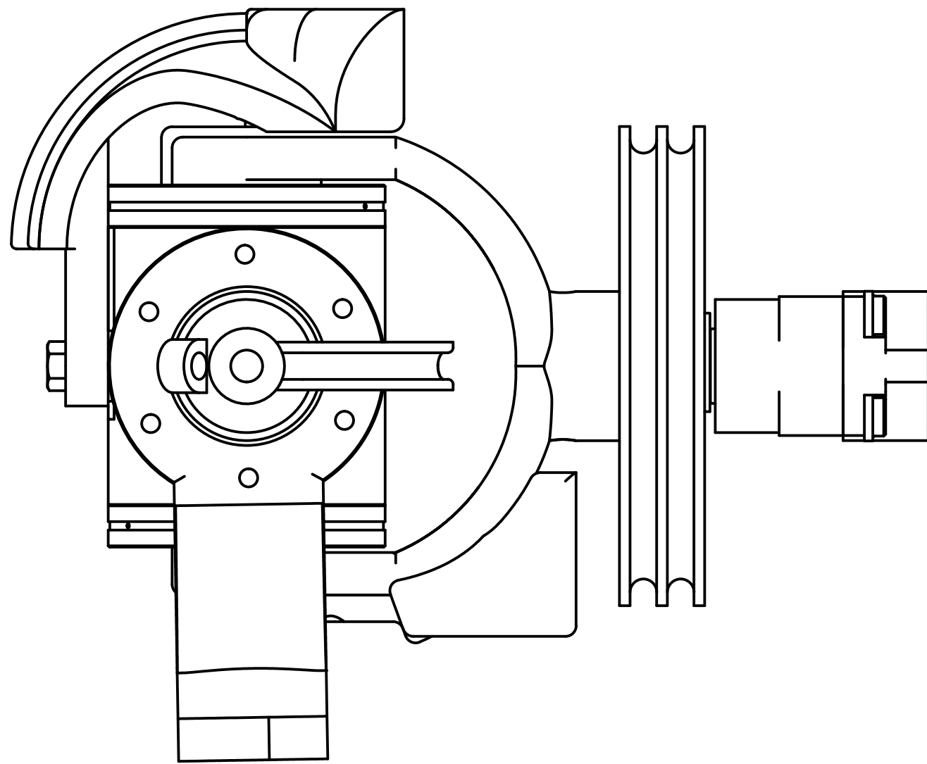
SIDE VIEW
